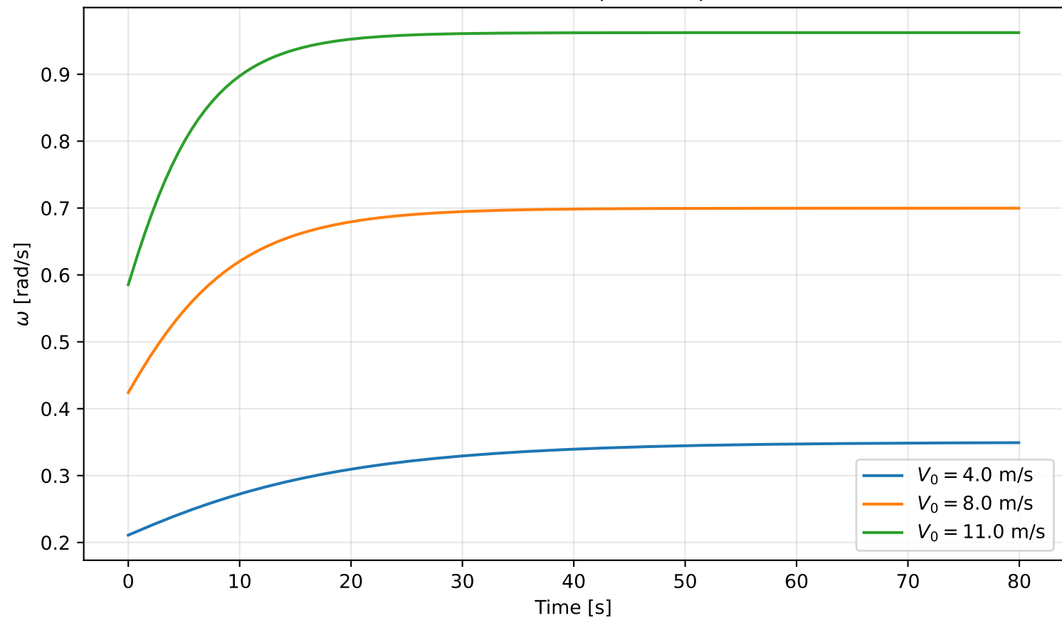
Below-rated rotor-speed response
